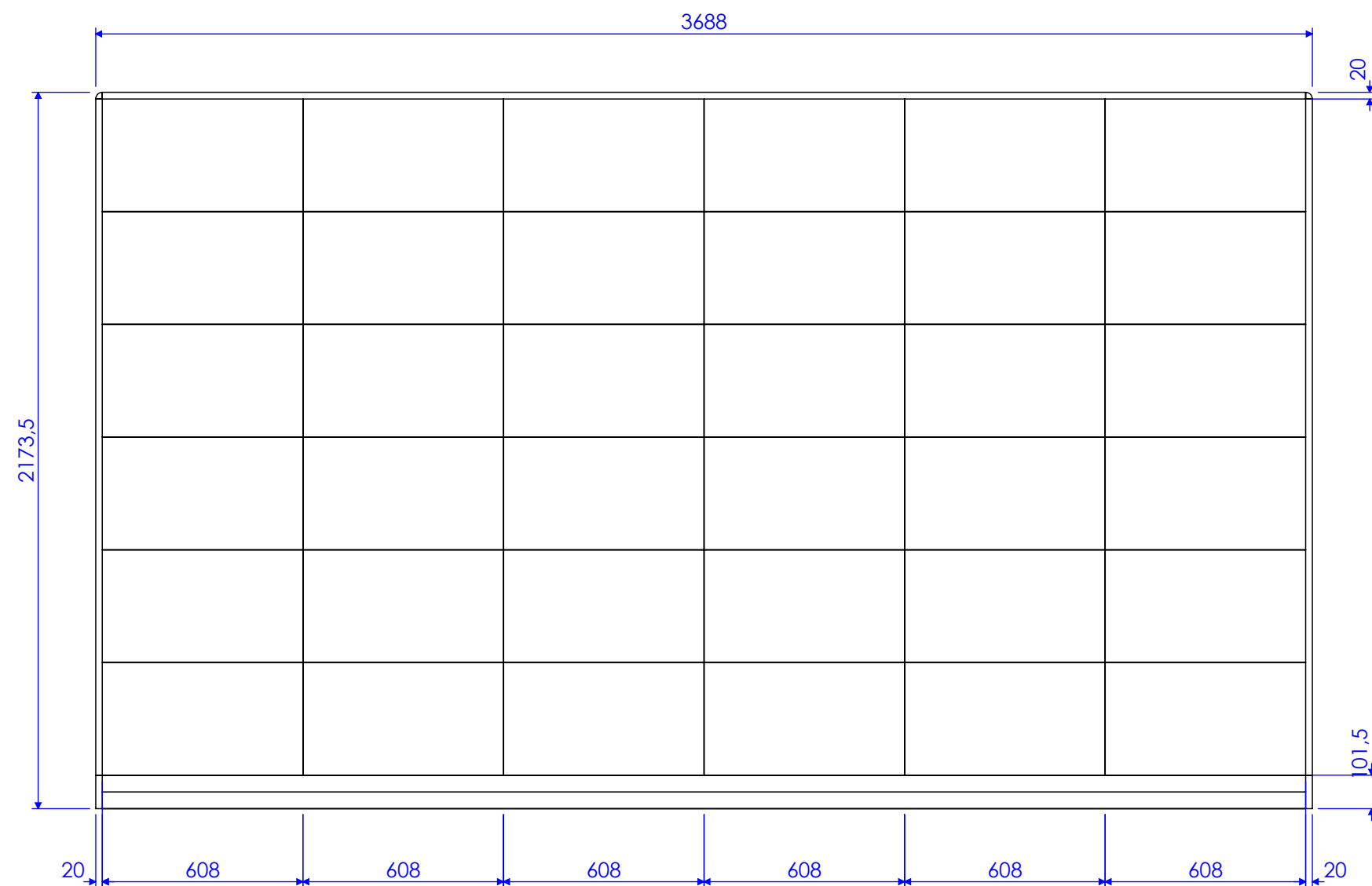
FRONT VIEW
